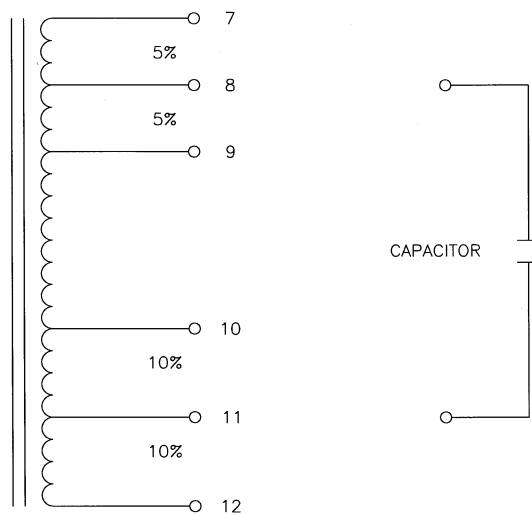
Fig. 9.3 Ferroresonant Transformer Capacitor Winding
